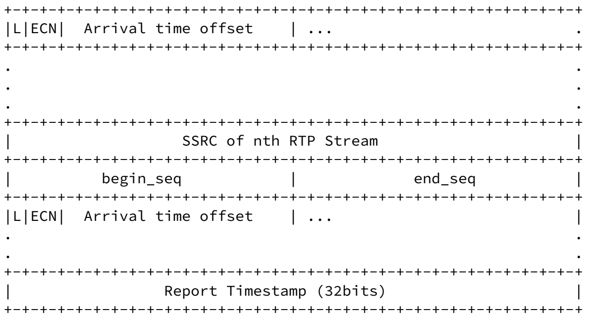
Figure 1: RTCP Congestion Control Feedback Packet Format
