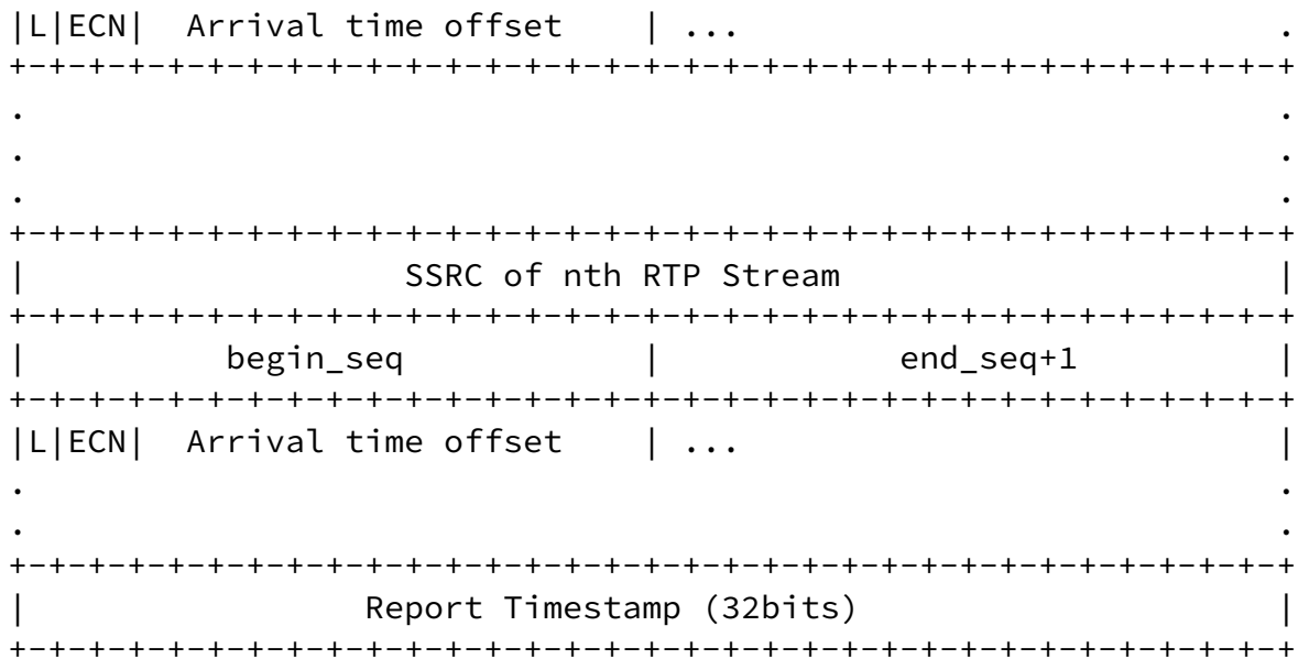
Figure 1: RTCP Congestion Control Feedback Packet Format
