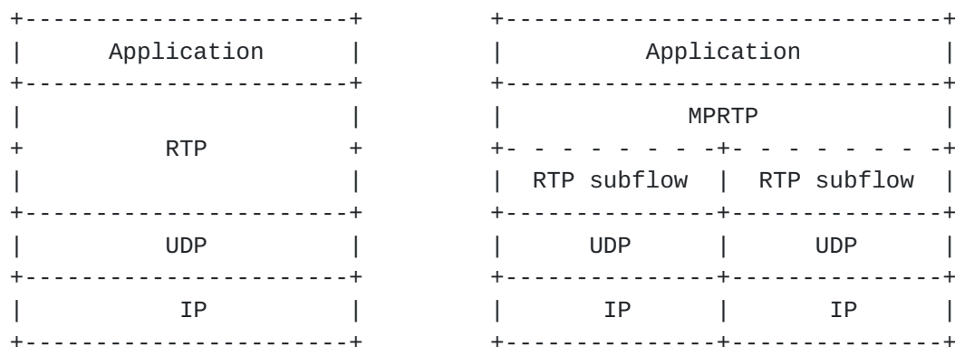
Figure 2: MPRTTP Architecture
