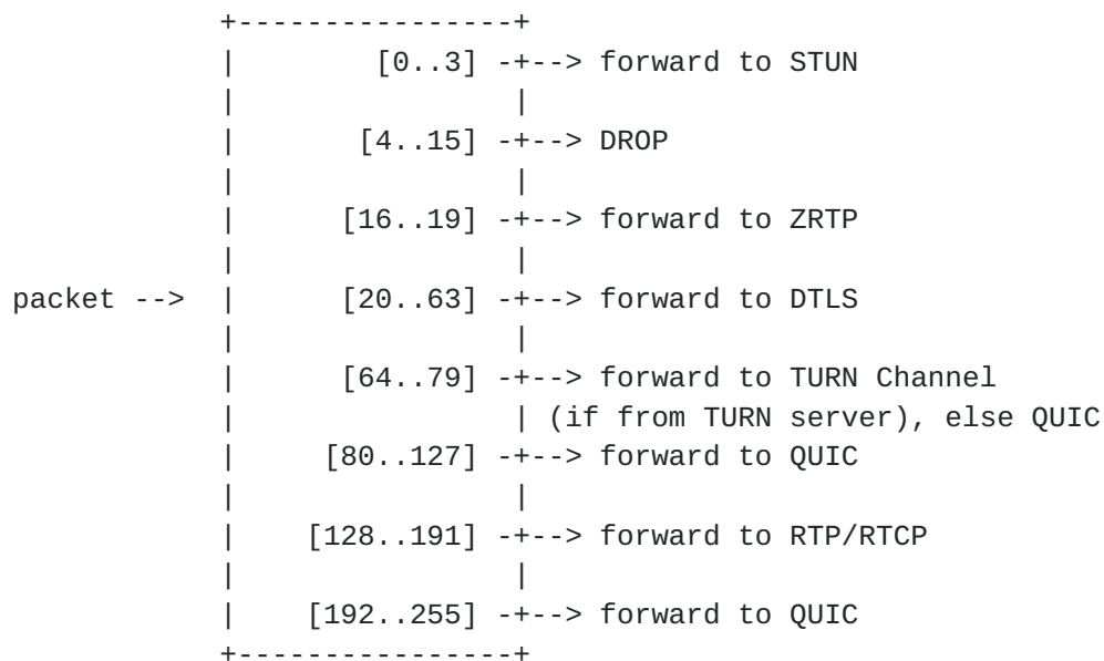
Figure 3: The receiver's packet demultiplexing algorithm.
