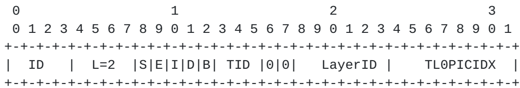
Long Frame Marking RTP Extension for [VVC]
