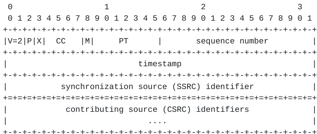
RTP Header According to [RFC3550]
