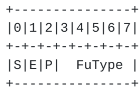
The Structure of FU Header
