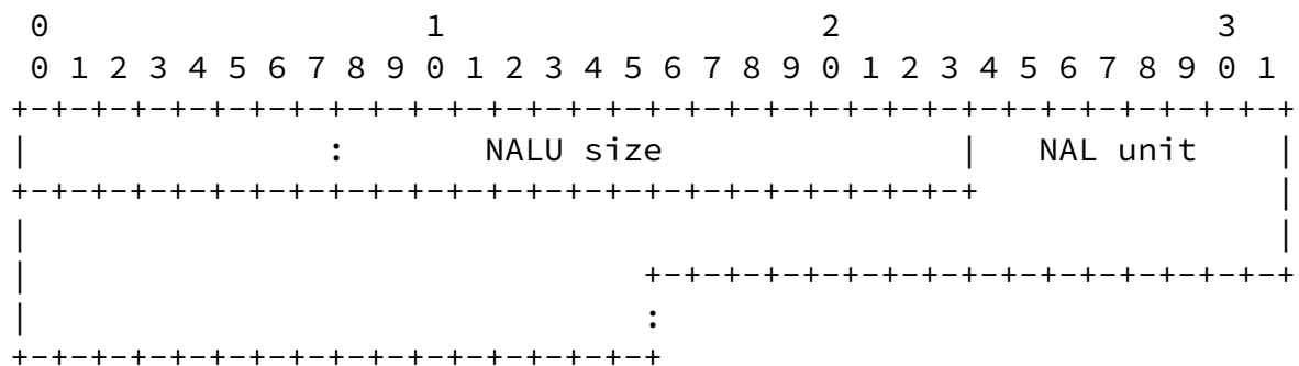
The Structure of an Aggregation Unit That Is Not the First Aggregation Unit in an AP
