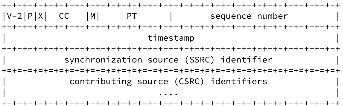
RTP Header According to [RFC3550]
