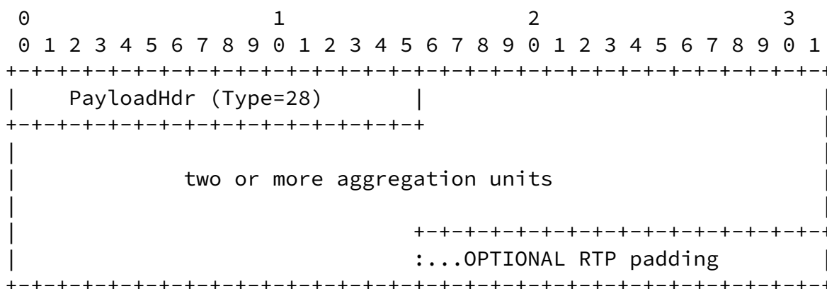
The Structure of an Aggregation Packet
