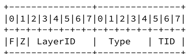
The Structure of the VVC NAL Unit Header.
