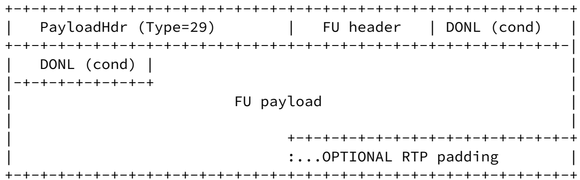
The Structure of an FU
