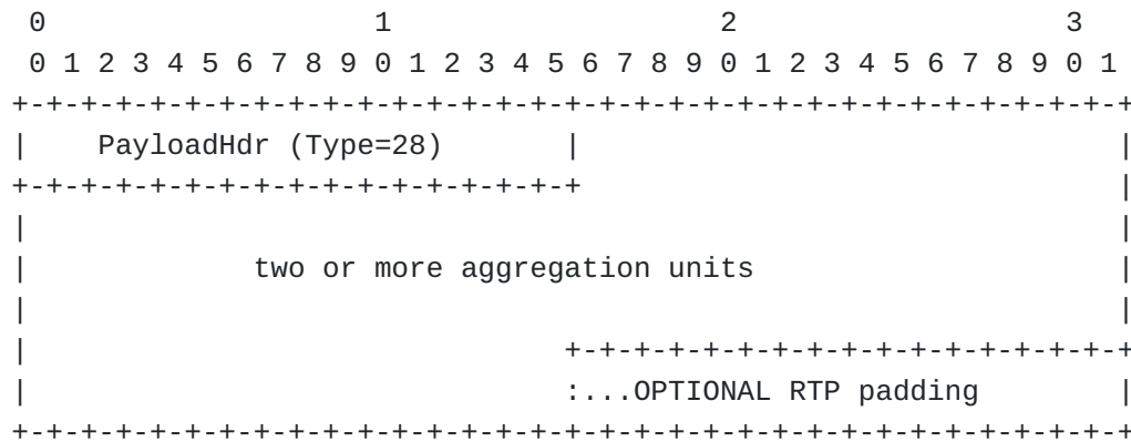
The Structure of an Aggregation Packet
