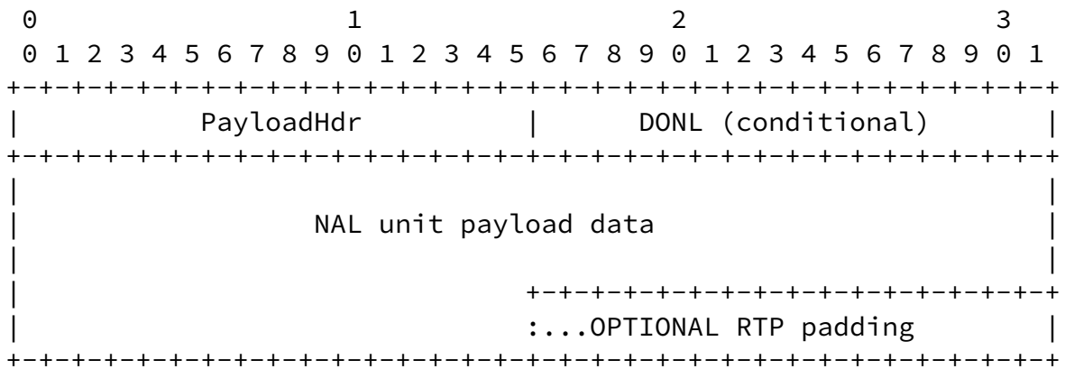
The Structure of a Single NAL Unit Packet
