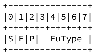
The Structure of FU Header
