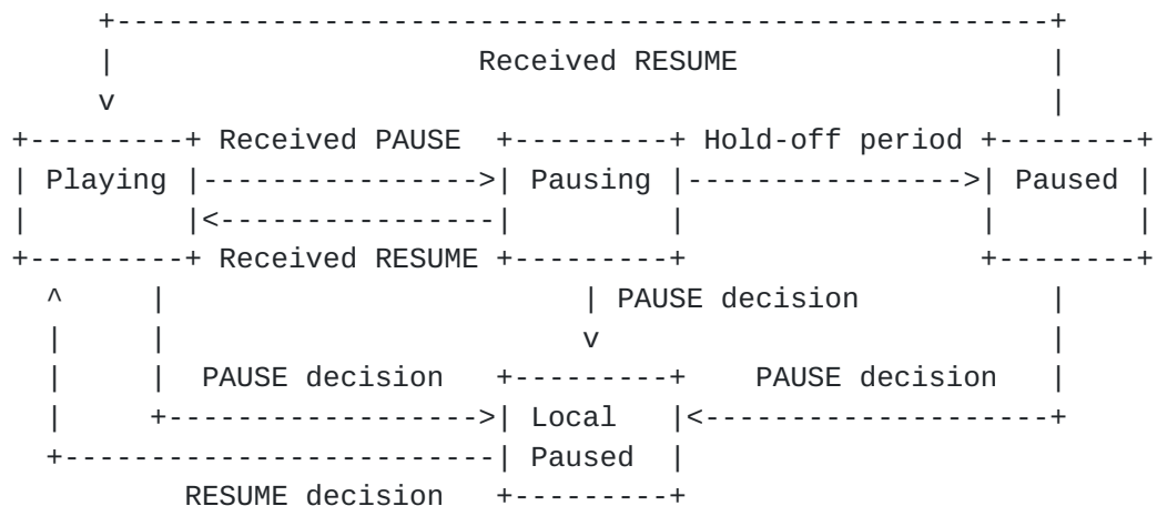
Figure 4: RTP Pause States
