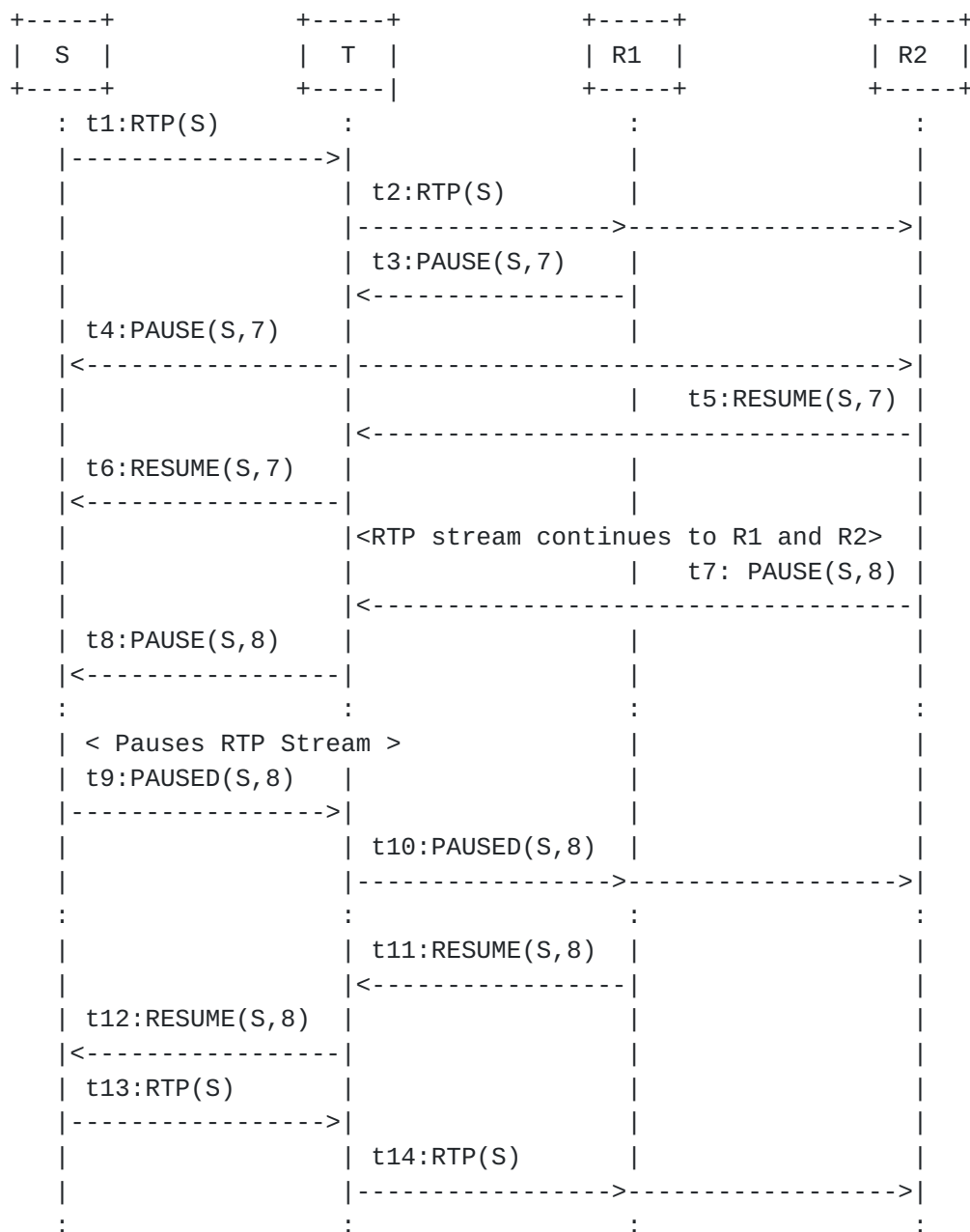
Figure 18: Pause and Resume Operation Between One Sender and Two Receivers Through Translator
