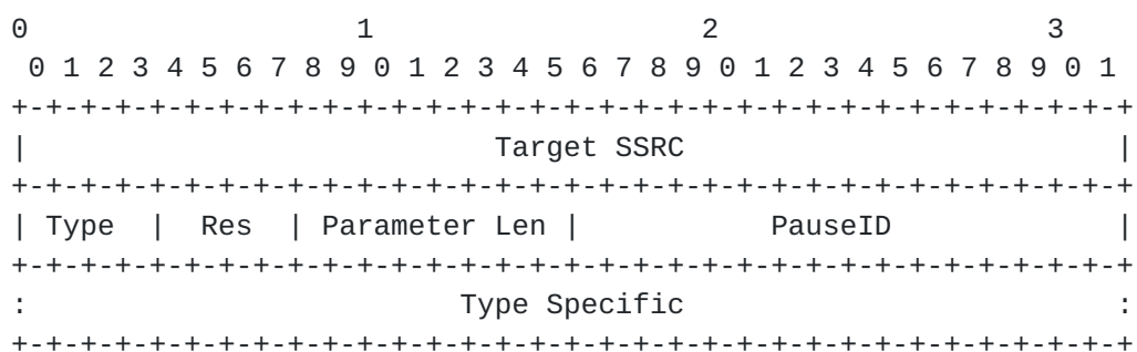
Figure 5: Syntax of FCI Entry in the PAUSE and RESUME message
