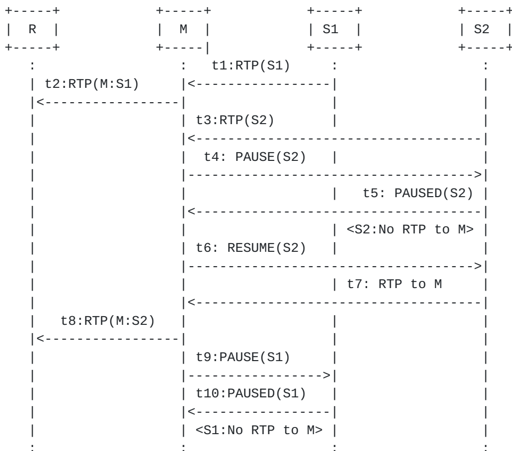
Figure 16: Pause and Resume Operation for a Voice Activated Mixer
