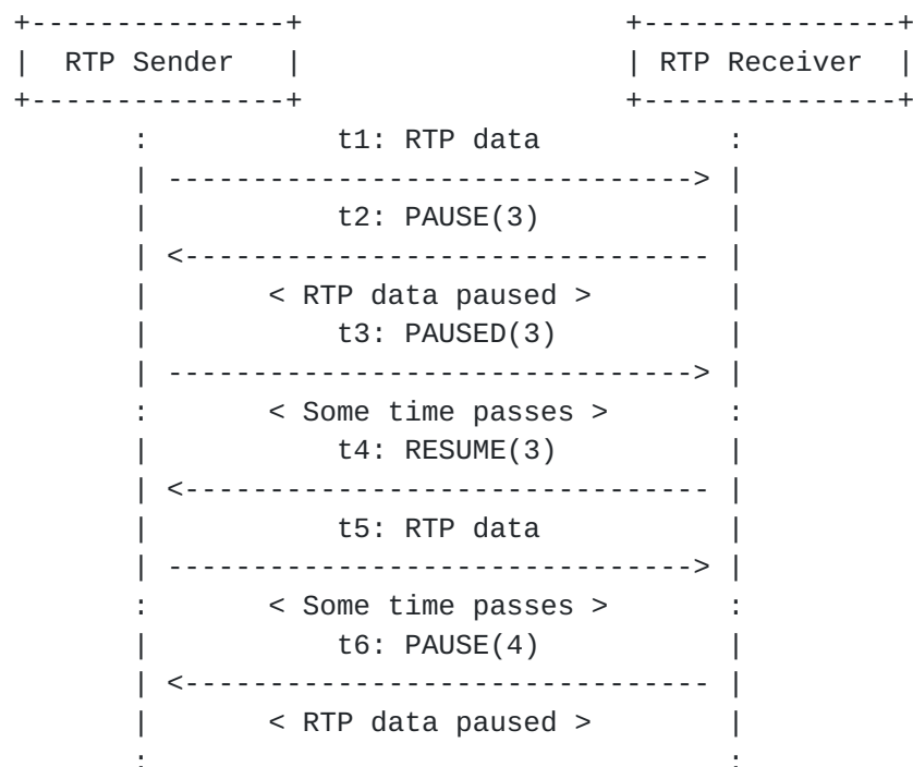
Figure 11: Pause and Resume Operation in Point-to-Point
