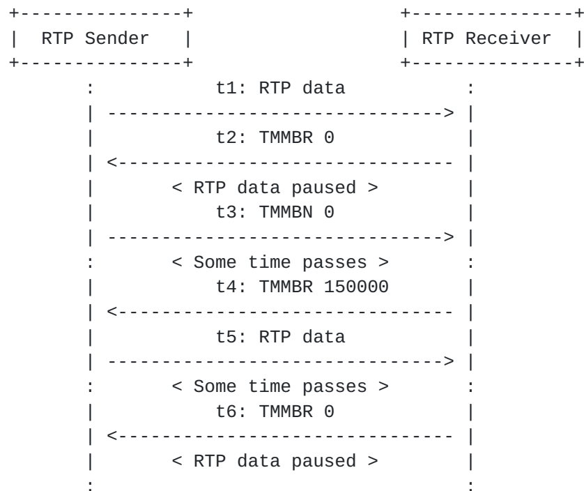
Figure 12: TMMBR Pause and Resume in Point-to-Point
