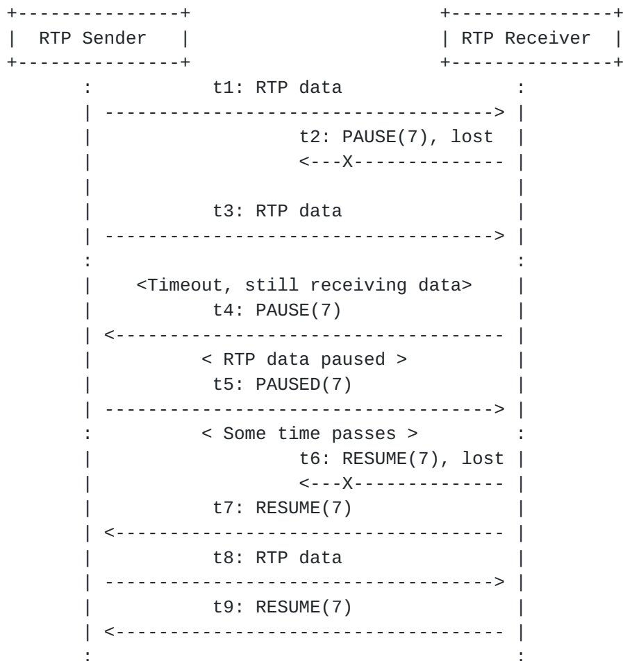
Figure 14: Pause and Resume Operation With Messages Lost
