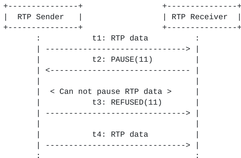
Figure 15: Pause Request is Refused in Point-to-Point
