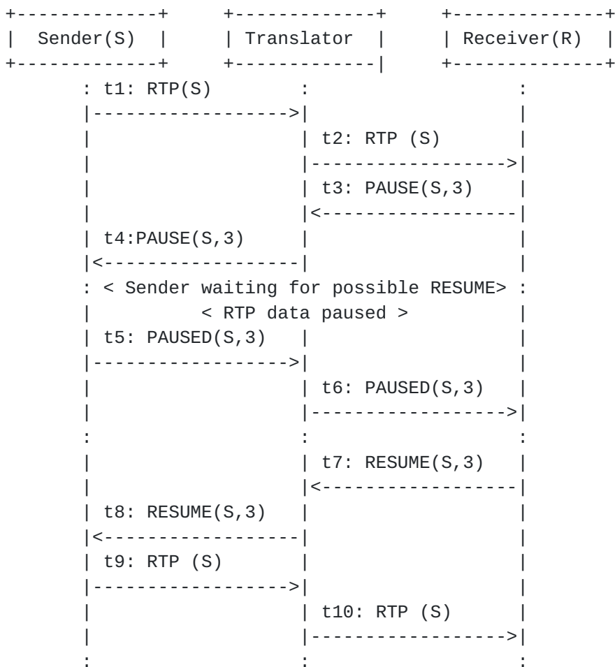
Figure 17: Pause and Resume Operation Between Two Participants Using a Translator
