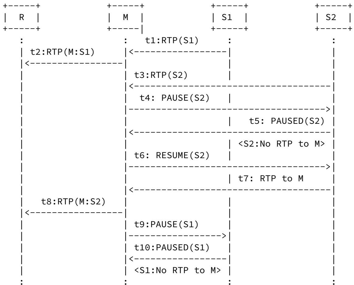
Figure 16: Pause and Resume Operation for a Voice Activated Mixer
