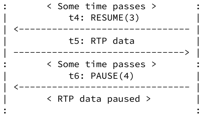
Figure 11: Pause and Resume Operation in Point-to-Point
