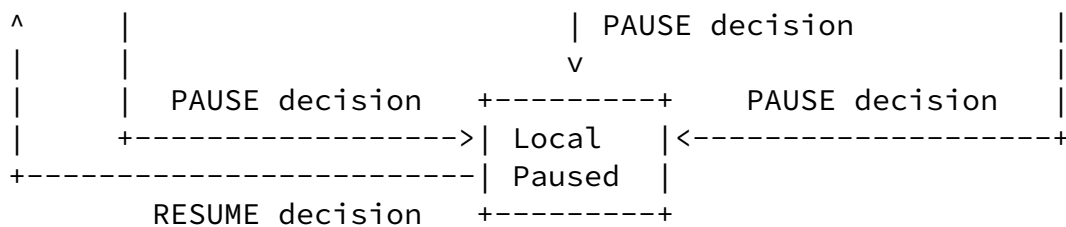
Figure 4: RTP Pause States
