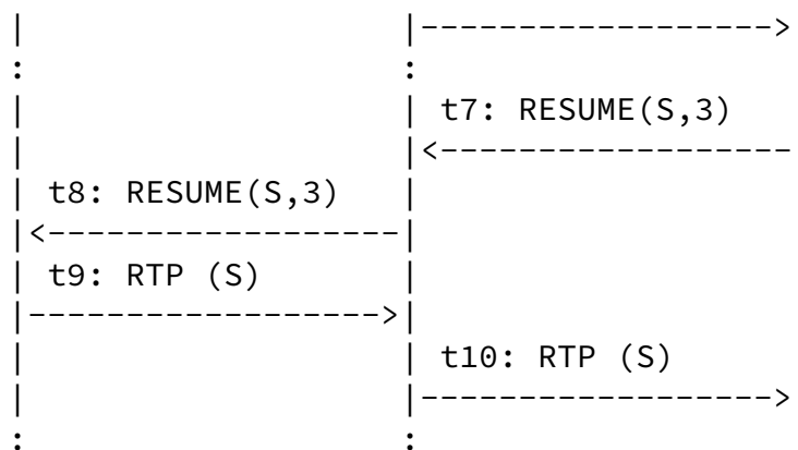
Figure 17: Pause and Resume Operation Between Two Participants Using a Translator
