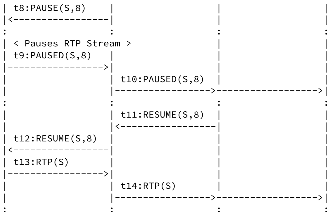
Figure 18: Pause and Resume Operation Between One Sender and Two Receivers Through Translator
