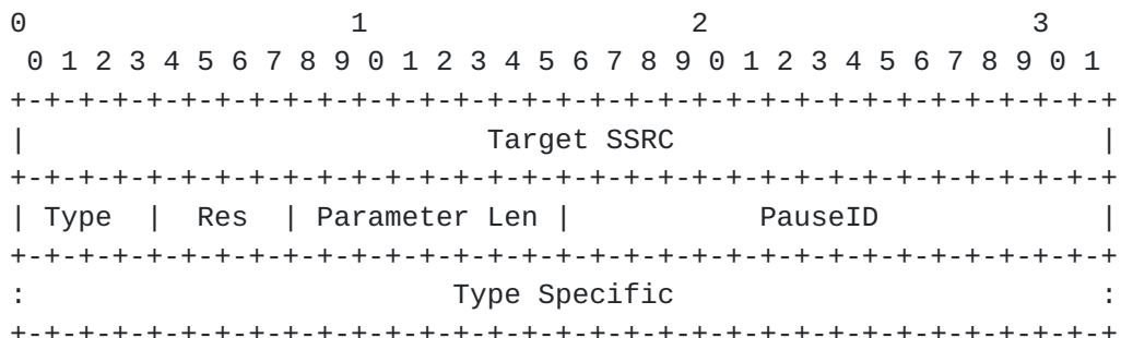
Figure 5: Syntax of FCI Entry in the PAUSE and RESUME message
