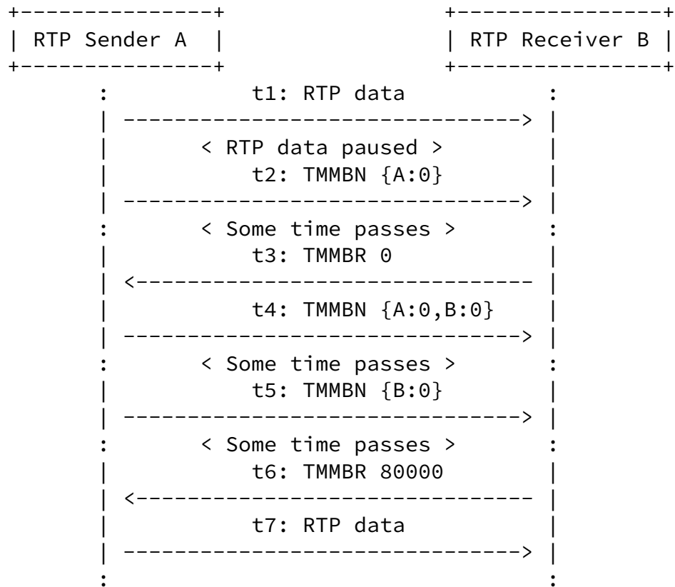
Figure 13: Unsolicited PAUSED using TMMBN
