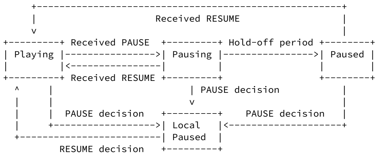
Figure 4: RTP Pause States
