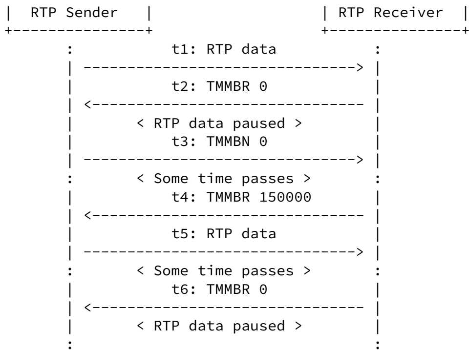
Figure 12: TMMBR Pause and Resume in Point-to-Point
