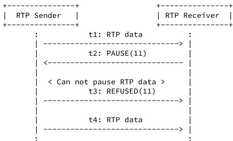
Figure 15: Pause Request is Refused in Point-to-Point
