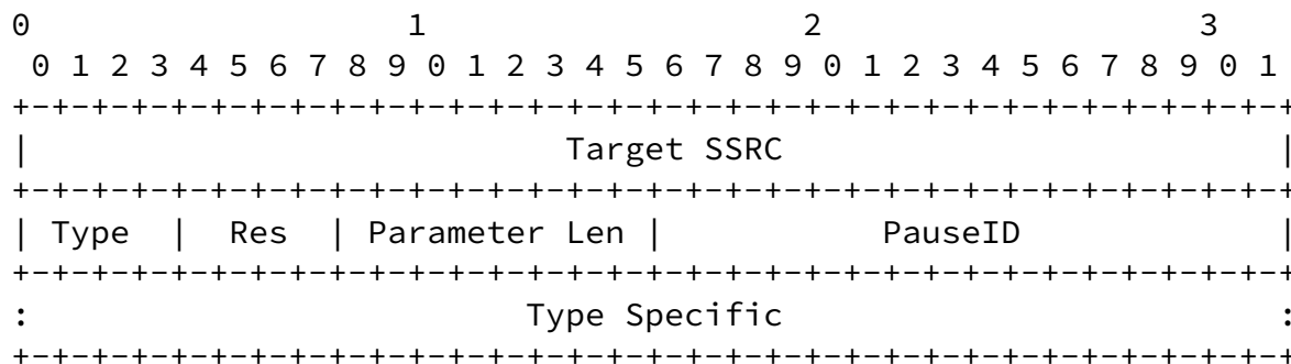
Figure 5: Syntax of FCI Entry in the PAUSE and RESUME message
