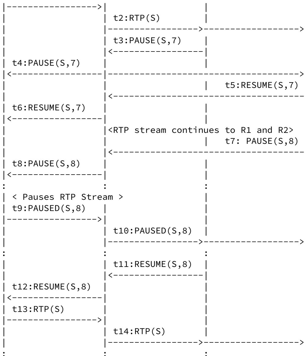
Figure 18: Pause and Resume Operation Between One Sender and Two Receivers Through Translator
