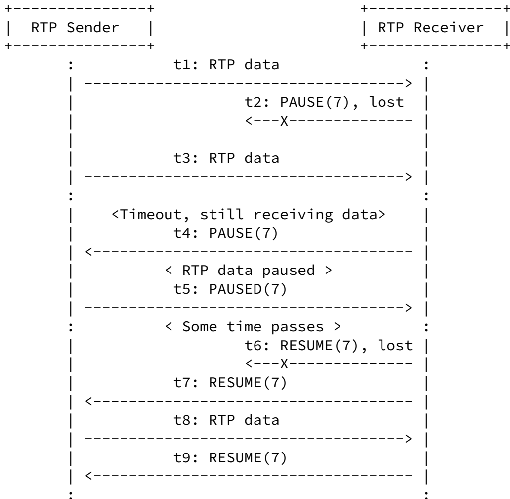
Figure 14: Pause and Resume Operation With Messages Lost
