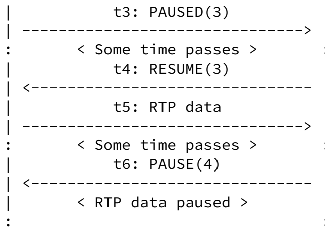
Figure 11: Pause and Resume Operation in Point-to-Point
