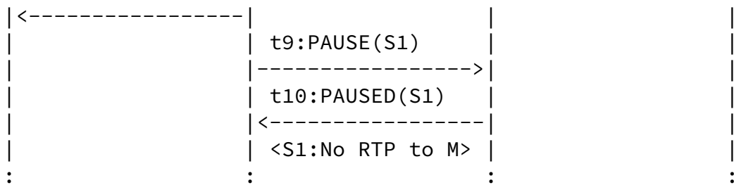
Figure 16: Pause and Resume Operation for a Voice Activated Mixer
