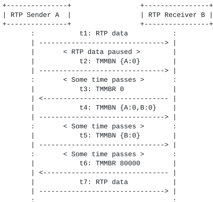
Figure 14: Unsolicited PAUSED using TMMBN
