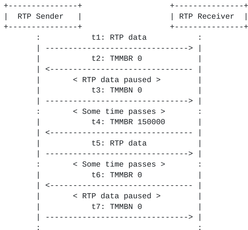
Figure 13: TMMBR Pause and Resume in Point-to-Point
