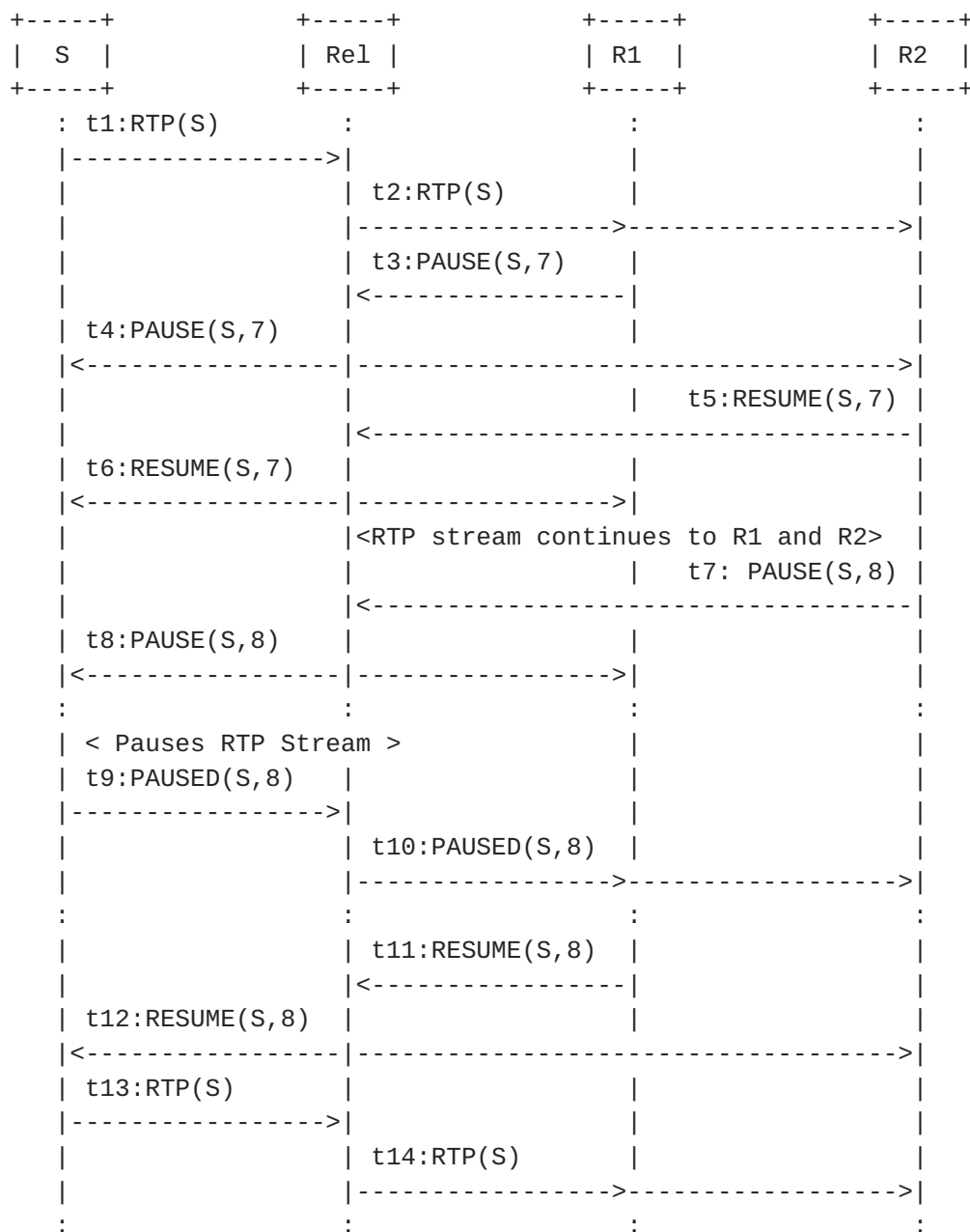
Figure 19: Pause and Resume Operation Between One Sender and Two Receivers Through Relay
