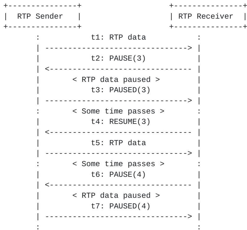
Figure 12: Pause and Resume Operation in Point-to-Point
