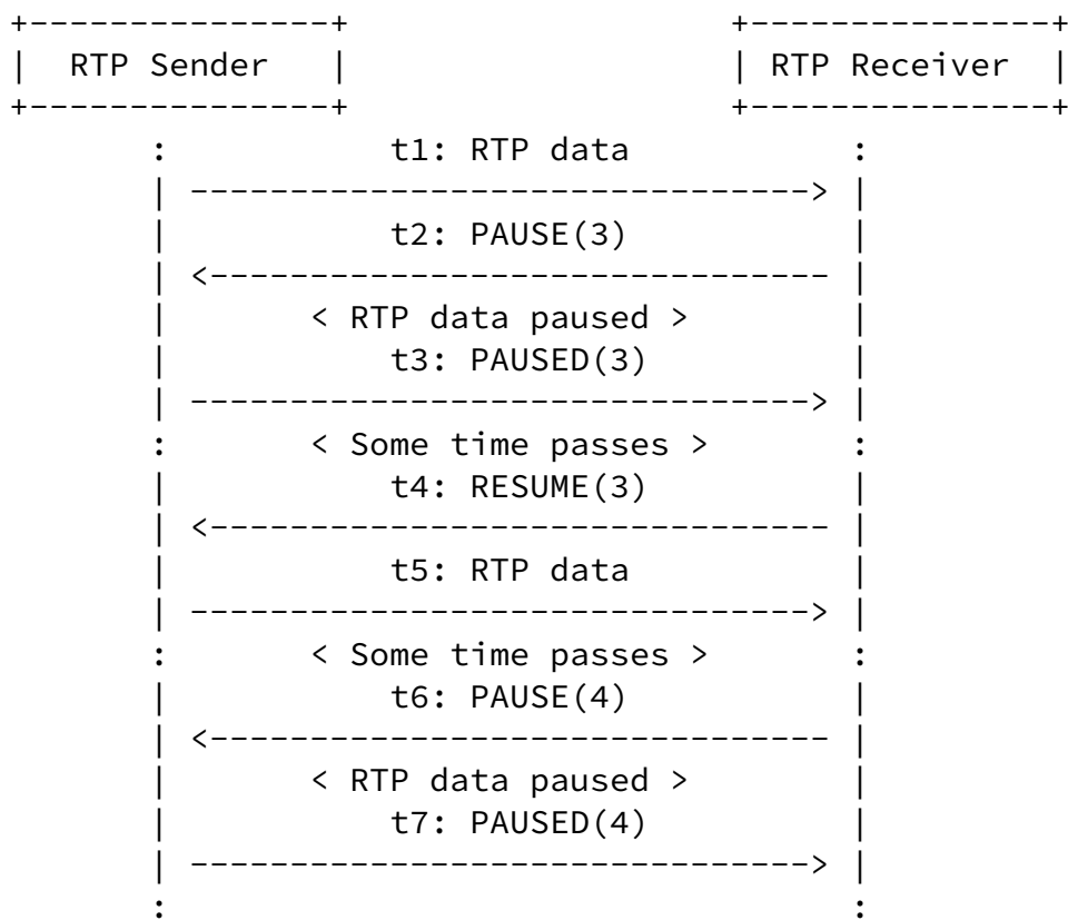
Figure 12: Pause and Resume Operation in Point-to-Point
