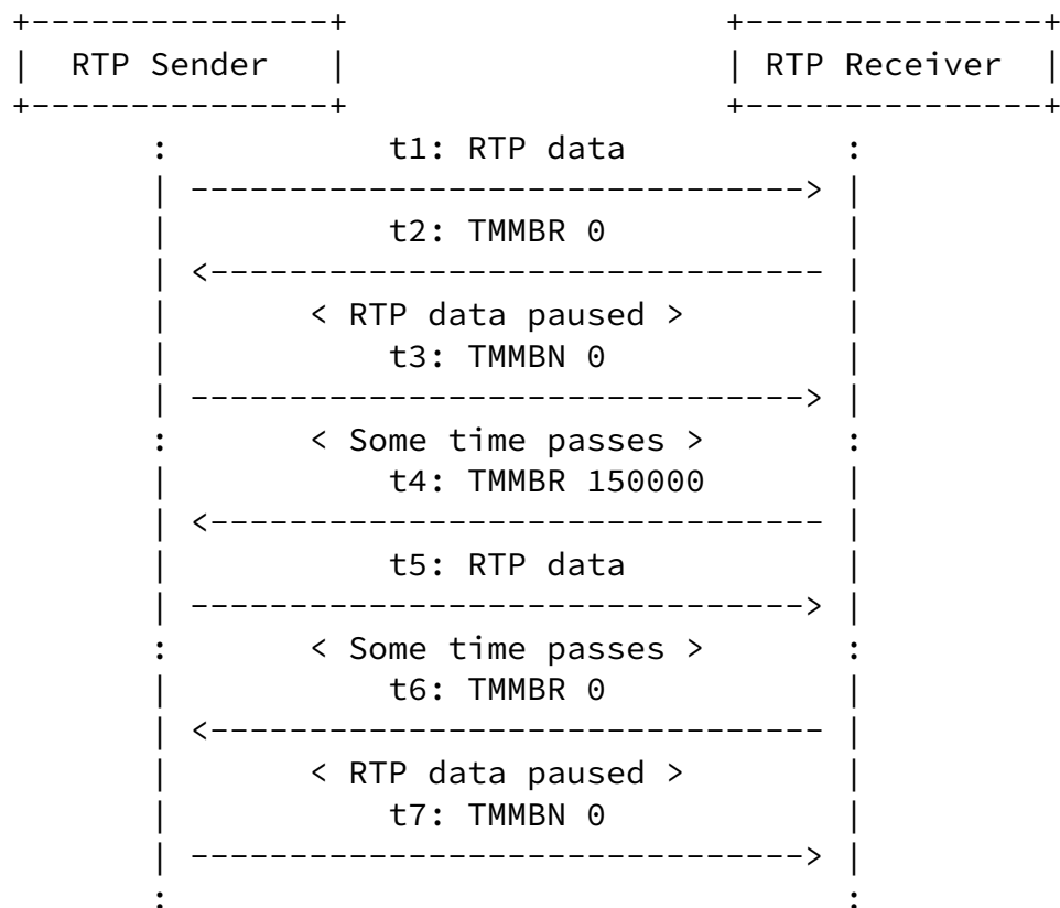
Figure 13: TMMBR Pause and Resume in Point-to-Point
