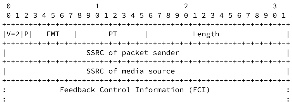
Figure 5: AVPF Common Feedback Message Packet Format
