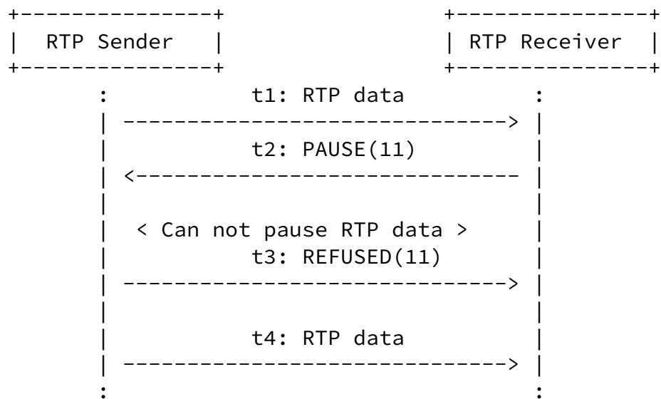
Figure 16: Pause Request is Refused in Point-to-Point
