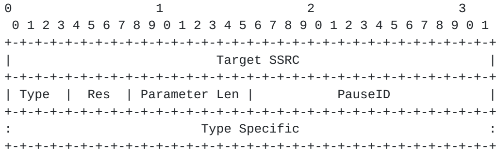
Figure 6: Syntax of FCI Entry in the PAUSE and RESUME message
