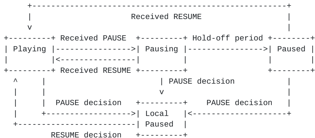
Figure 4: RTP Pause States in Sender
