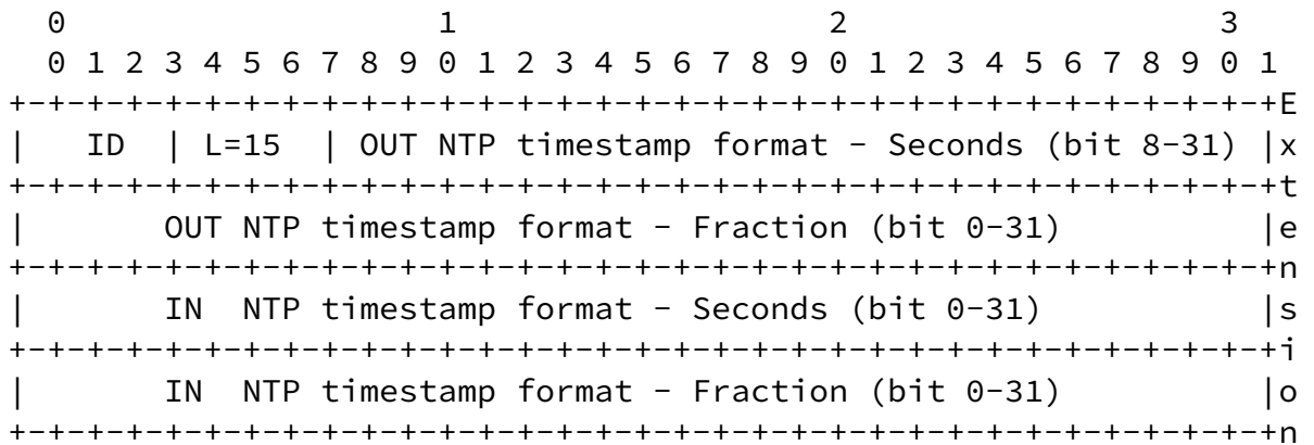
Figure 1: Splicing Interval Using the One-Byte Header Format
