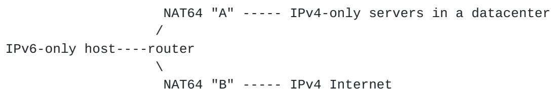
Figure 2: NAT64s with Assisting Router
