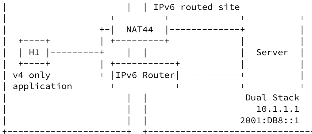
Figure 5: Network Scenario #2
