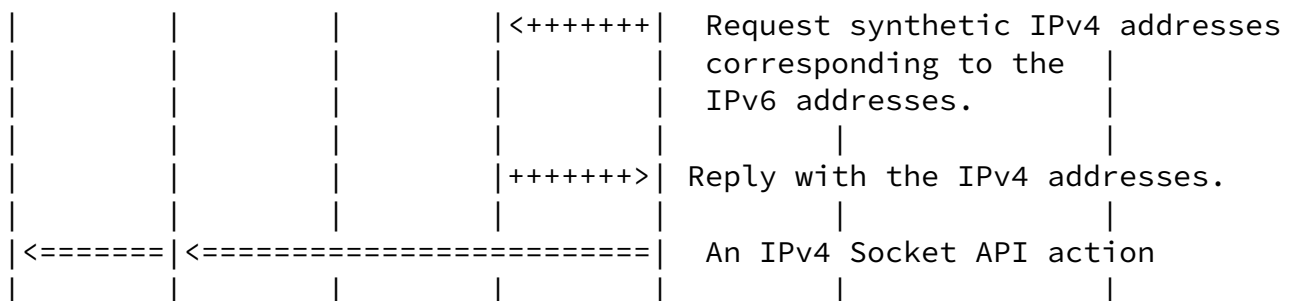
Figure 6: Example of BIH as API addition
