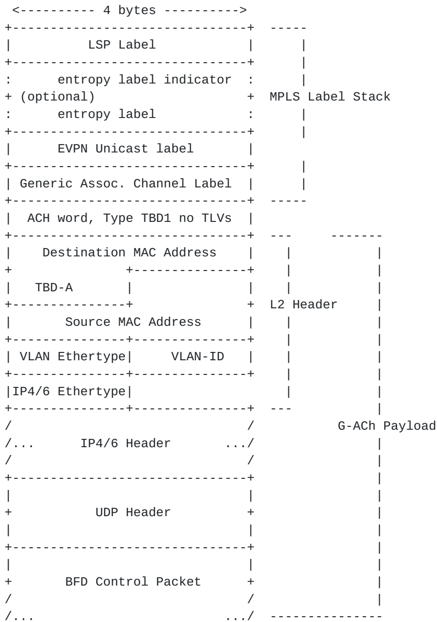
Figure 1. MPLS Unicast Encapsulation
