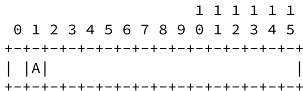
Figure 5 Bitmap field in the DF Election Extended Community
