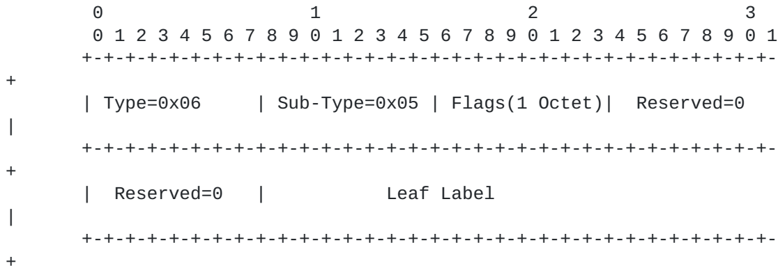
Figure 4: E-Tree Extended Community
