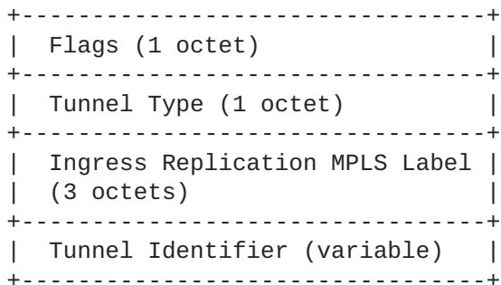
Figure 5: PMSI Tunnel Attribute
