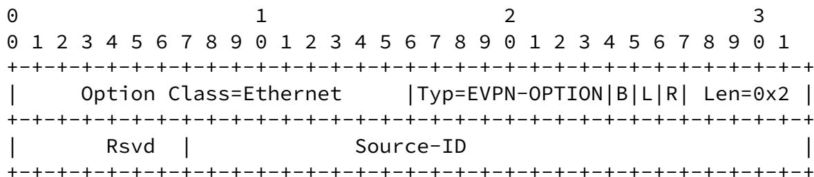
Figure 2: Ethernet Option TLV with ESI label
