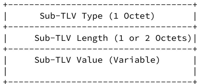
Figure 3: Geneve tunnel option types sub-TLV
