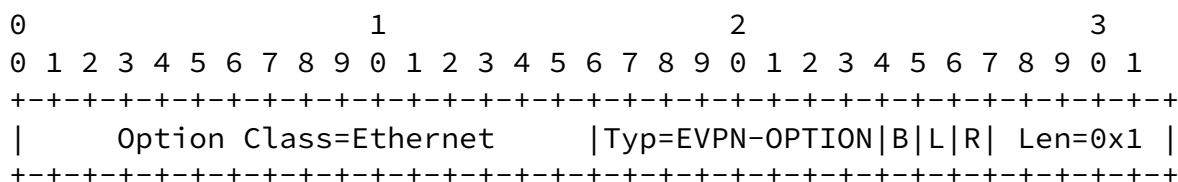
Figure 1: Ethernet Option TLV without ESI label
