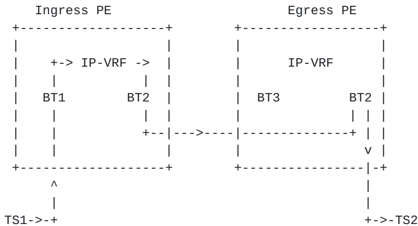
Figure 3: Asymmetric IRB
