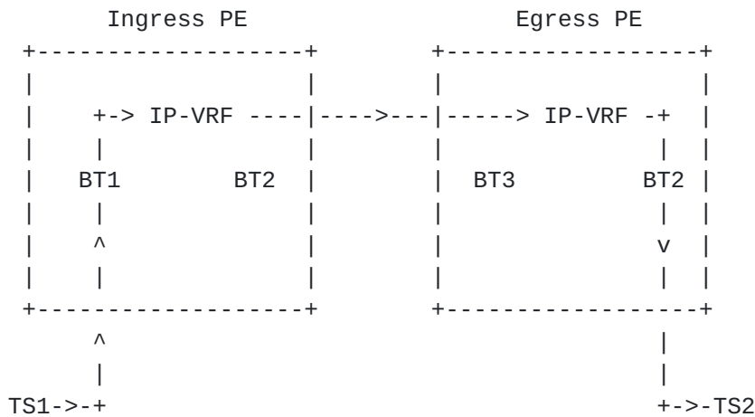
Figure 2: Symmetric IRB
