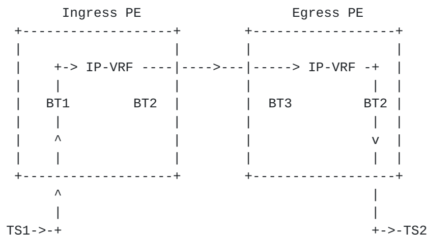
Figure 2: Symmetric IRB
