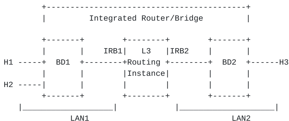
Figure 2: Integrated Router/Bridge
