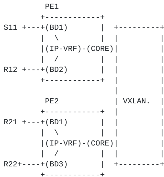
Figure 3 Intra-subnet bridging
