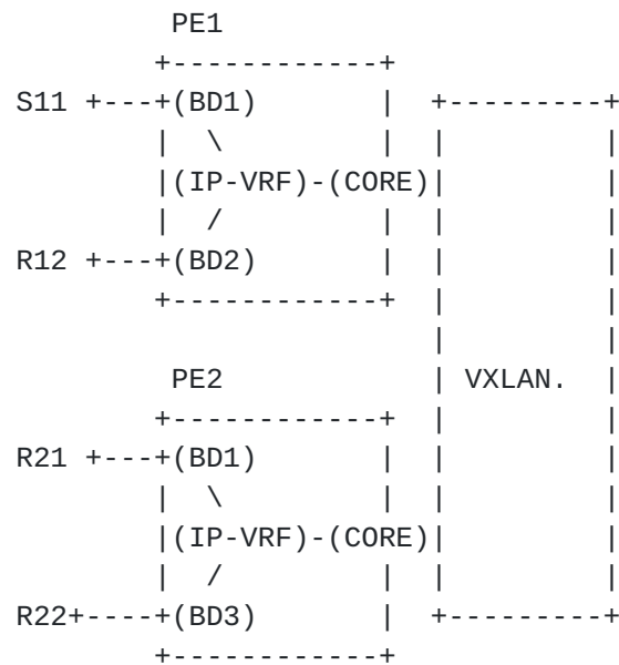
Figure 3 Intra-subnet bridging
