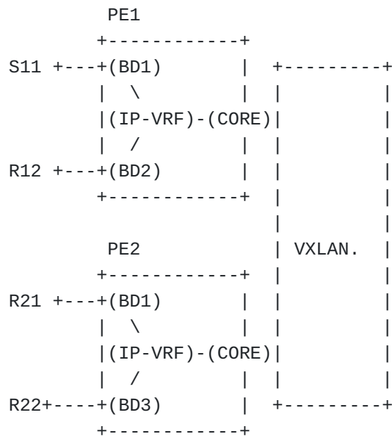
Figure 3: Intra-subnet bridging
