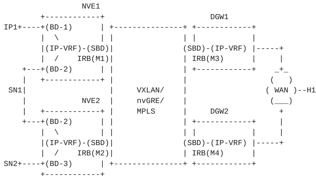
Figure 8 Interface-ful with unnumbered core-facing IRB model
