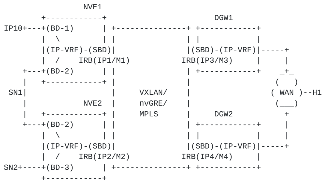
Figure 7 Interface-ful with core-facing IRB model
