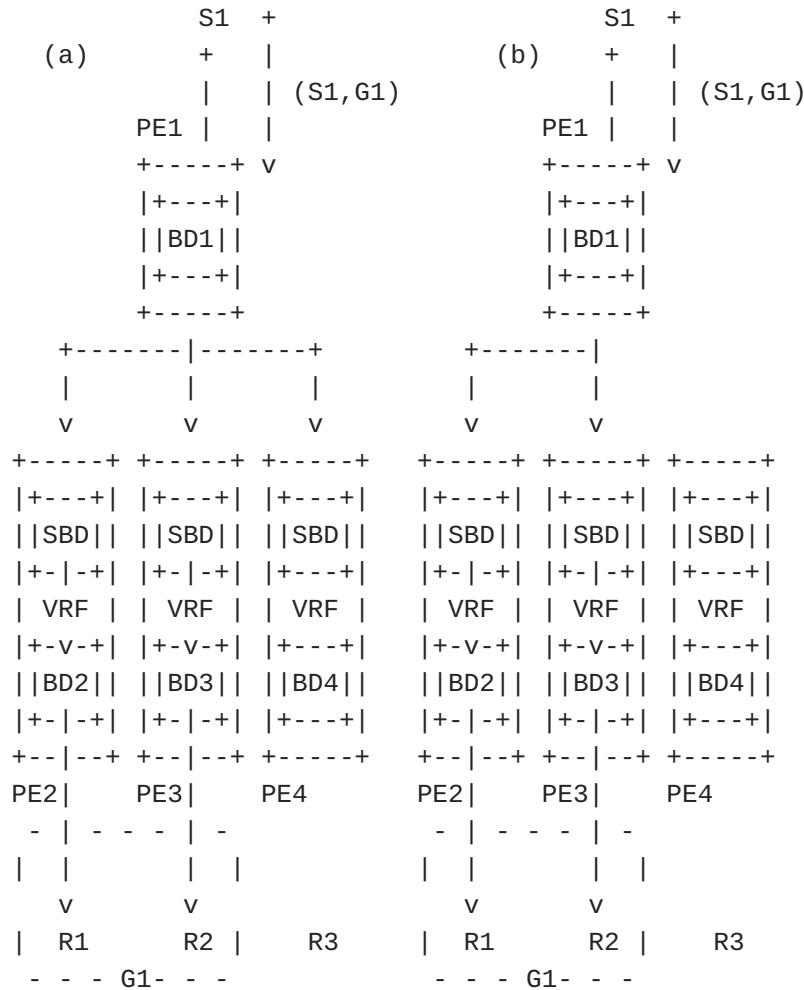
Figure 2: Inter-subnet IP Multicast
