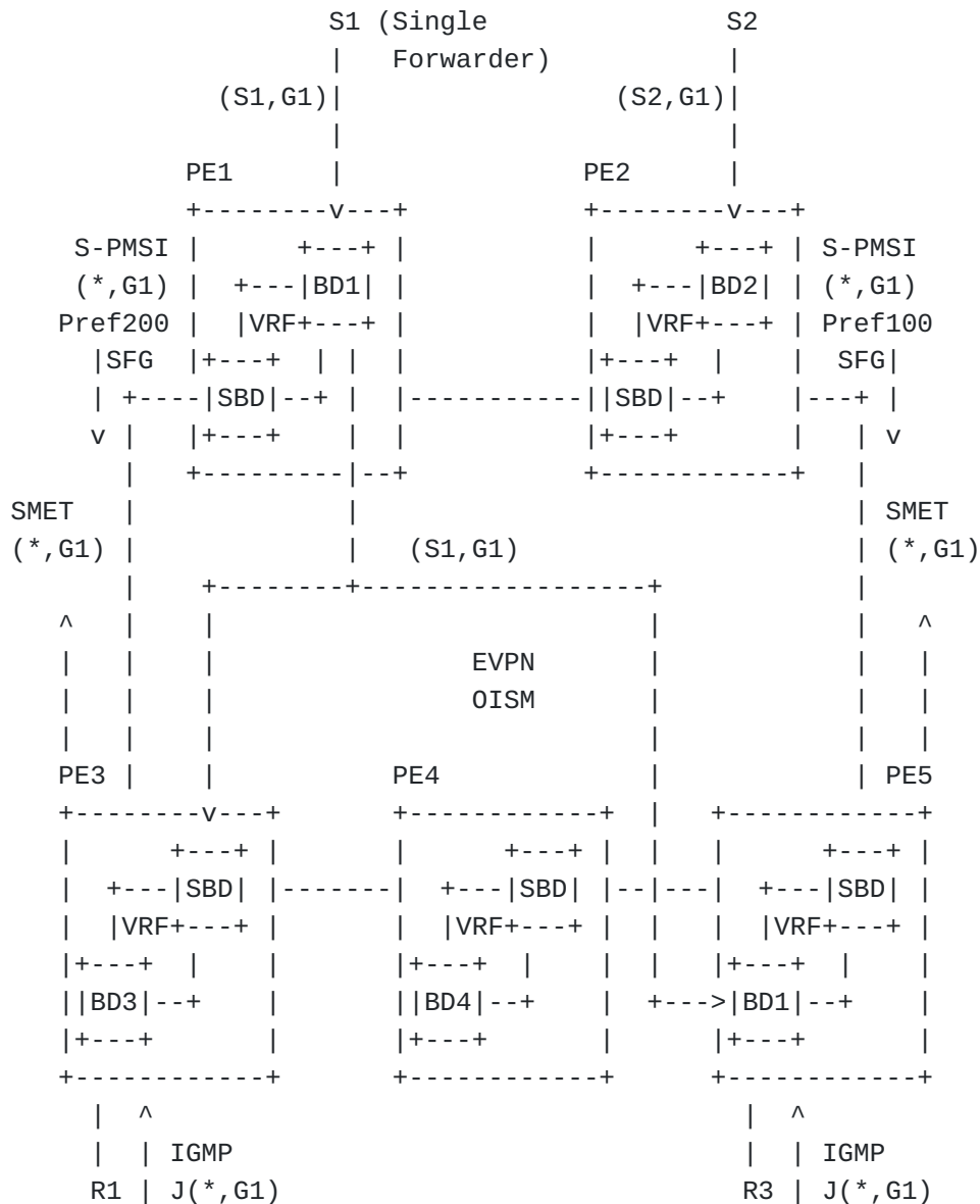
Figure 4: WS Solution for Redundant G-Sources
