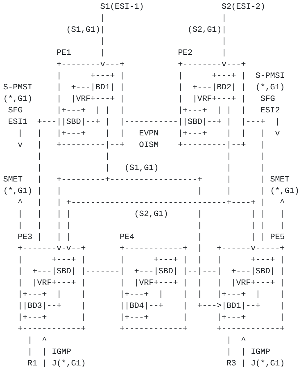
Figure 8: HS Solution for single-homed Redundant G-Sources in OISM
