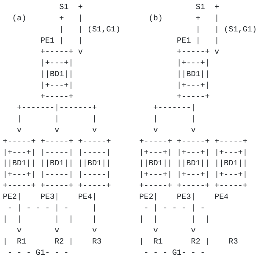
Figure 1: Intra-subnet IP Multicast
