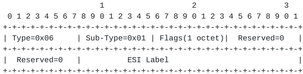
Figure 6: ESI Label Extended Community
