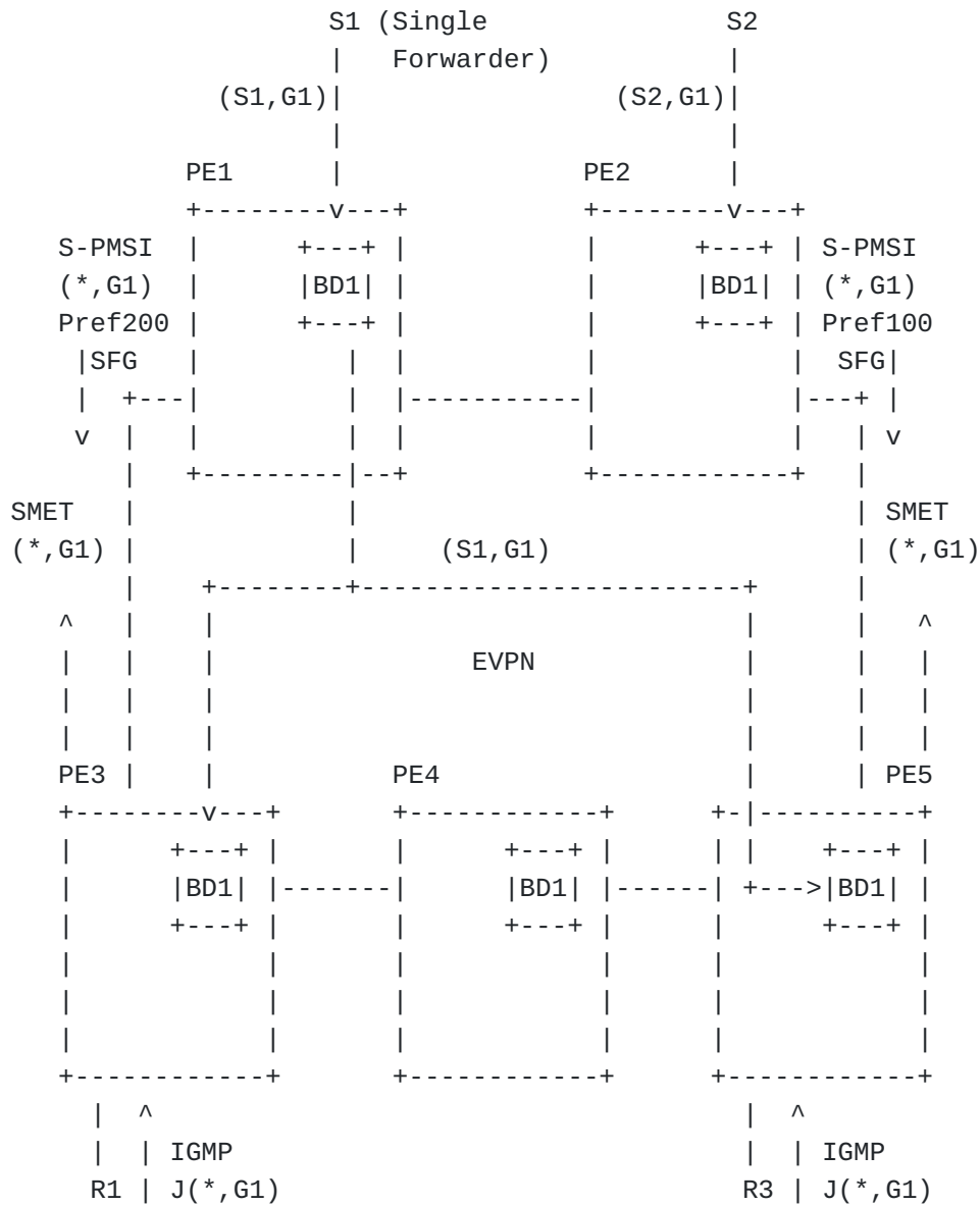
Figure 5: WS Solution for Redundant G-Sources in the same BD
