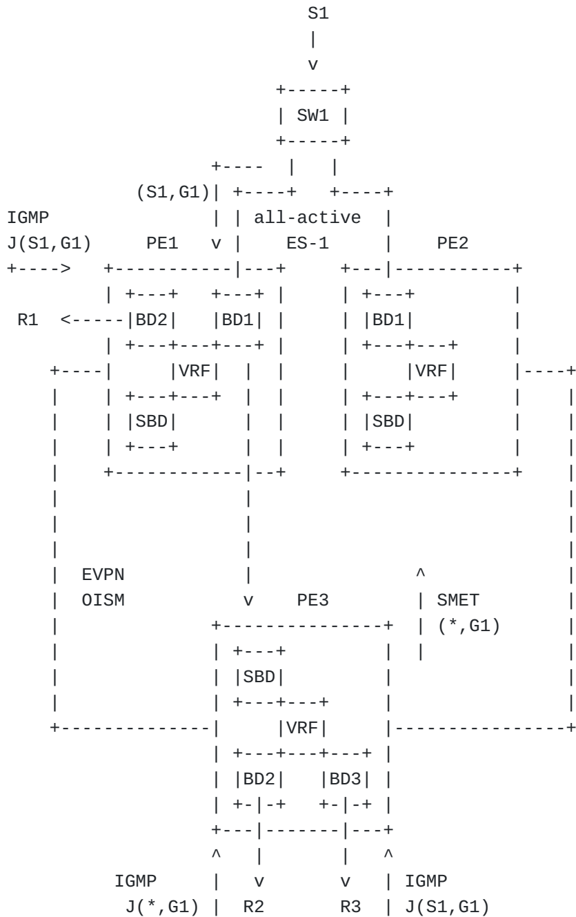
Figure 3: All-active Multi-homing and OISM
