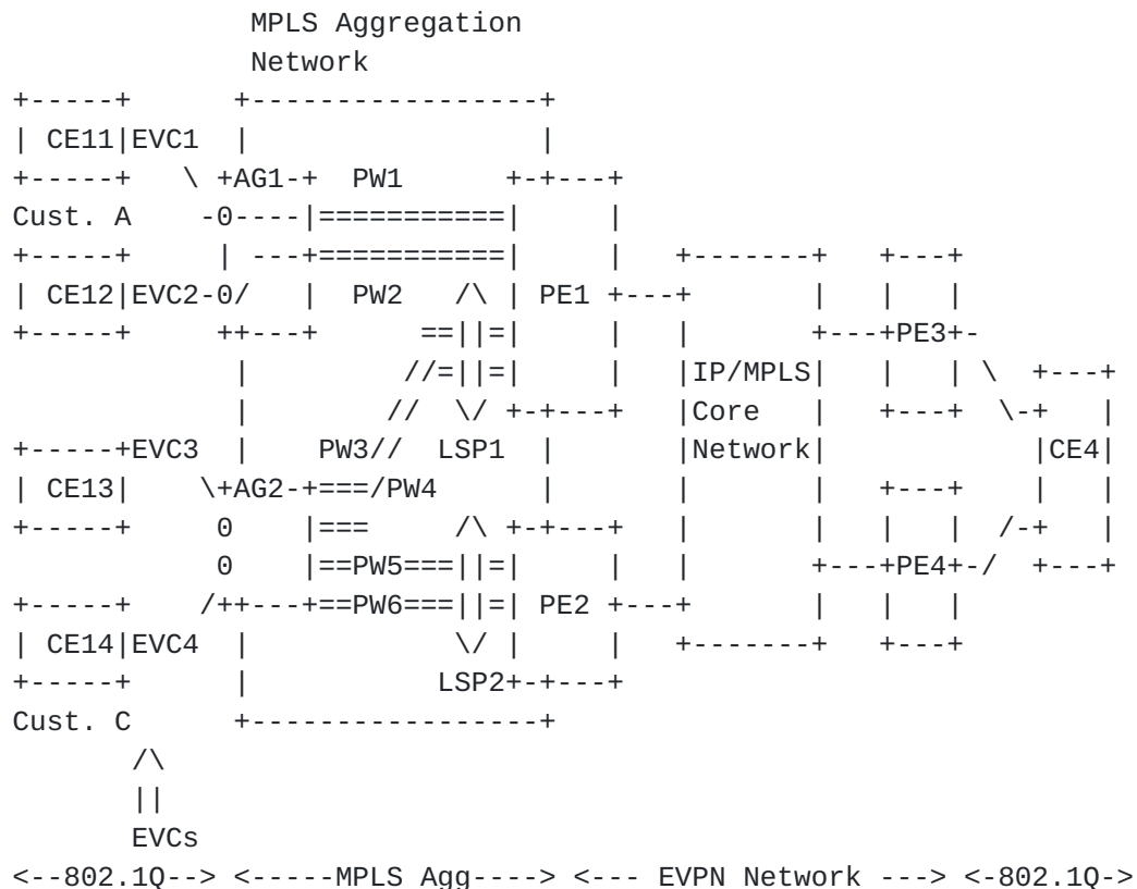
Figure 2: DHN and SH on MPLS Aggregation networks
