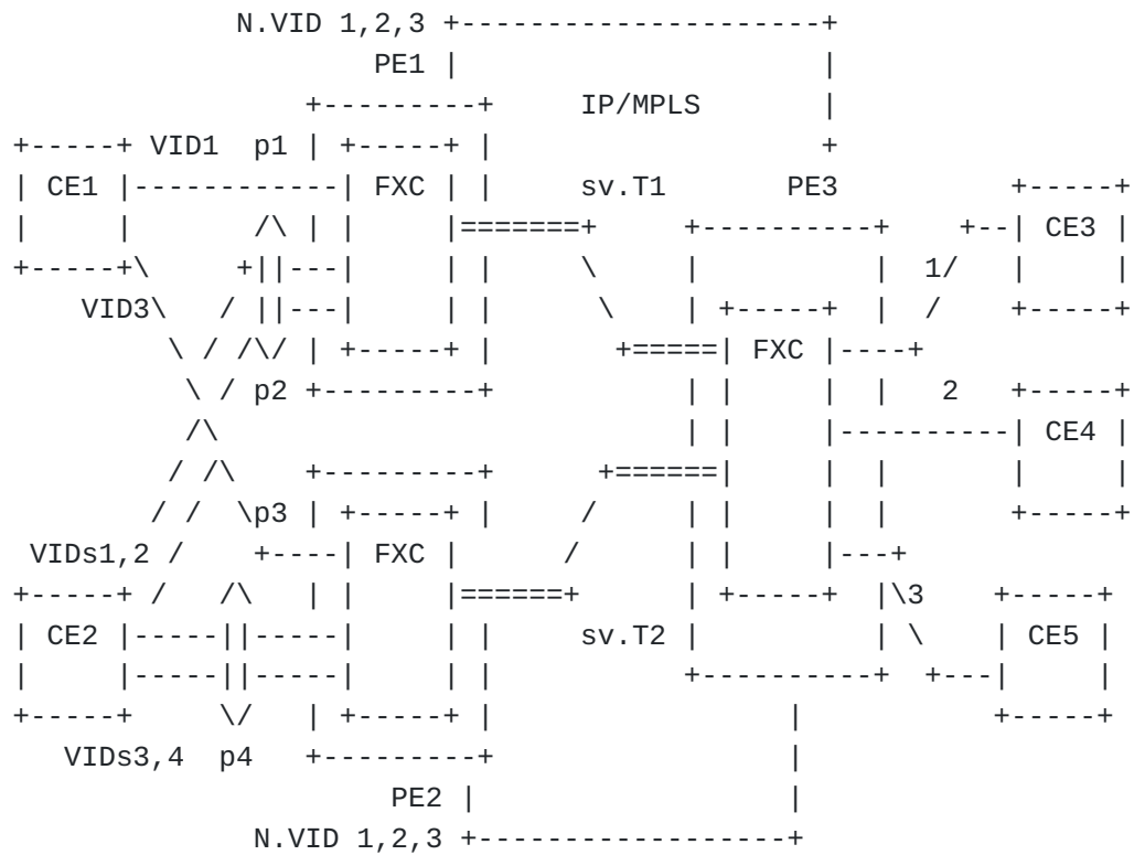
Figure 1: VLAN-Signaled Flexible Xconnect
