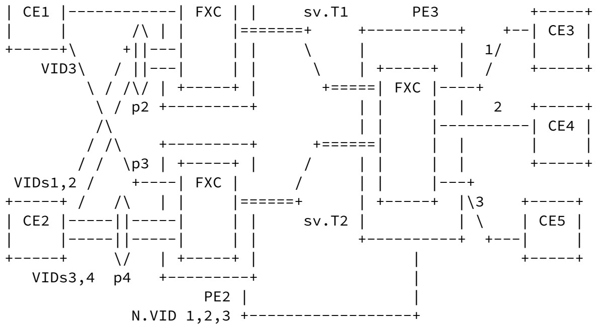
Figure 1: VLAN-Signaled Flexible Xconnect
