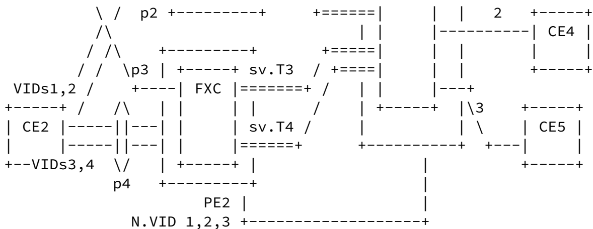
Figure 2: Default Flexible Xconnect
