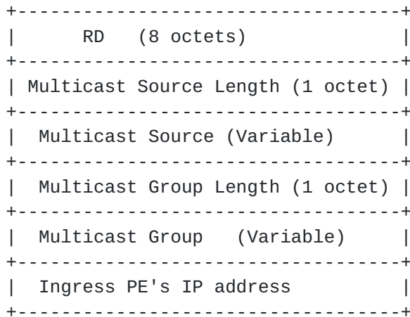
Figure 1: NLRI of S-PMSI A-D Route
