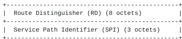
Figure 4: SFPR Route Type Specific NLRI
