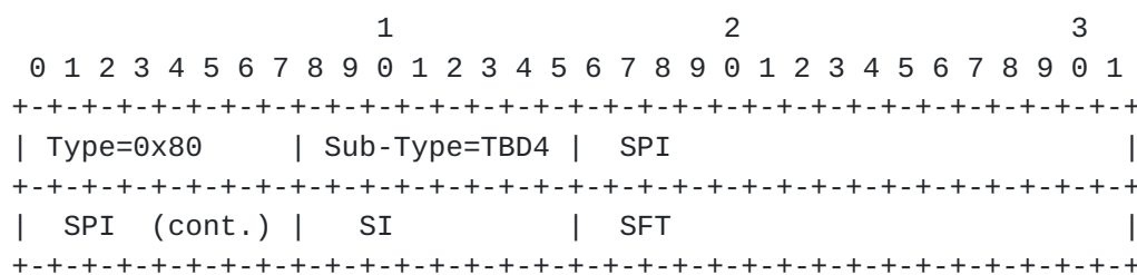
Figure 10: The Format of the Flow Specification for SFC Classifiers Extended Community
