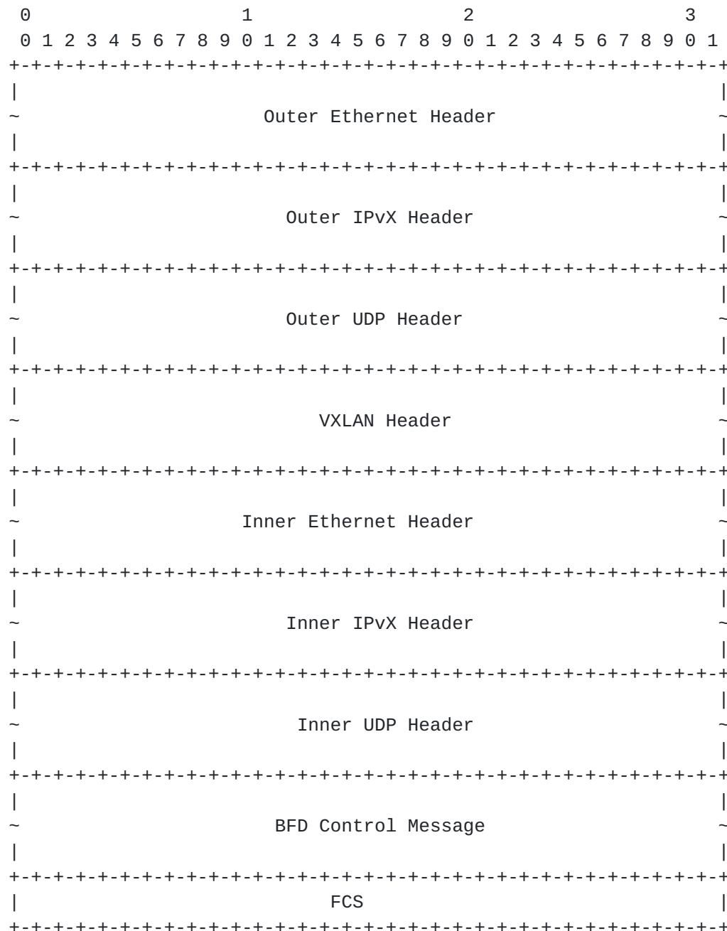
Figure 2: VXLAN Encapsulaion of BFD Control Message
