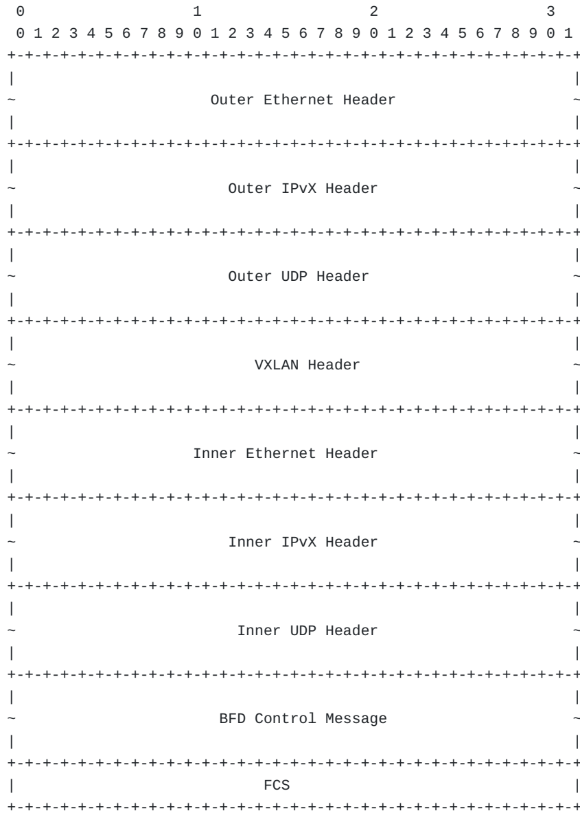
Figure 2: VXLAN Encapsulation of BFD Control Message
