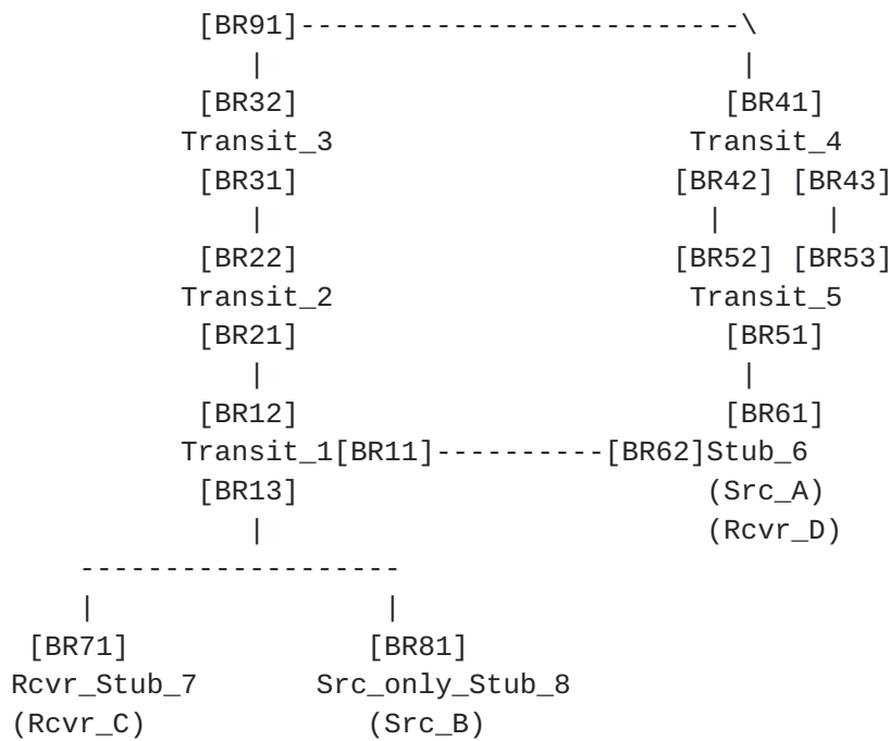
Figure 1: Example inter-domain topology. [BRXY] represents a BGMP border router. Transit_X is a transit domain network. *_Stub_X is a stub domain network.
