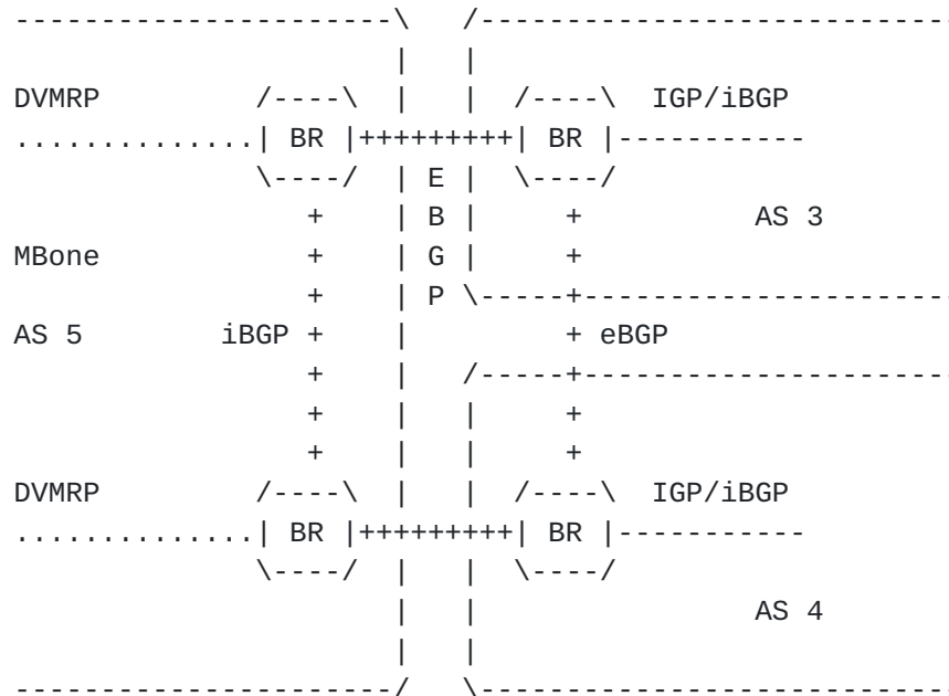
Figure 2: Preventing Transit through MBone Stub
