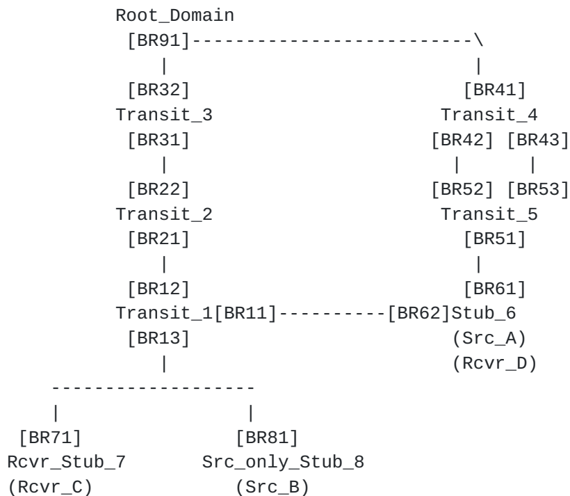
Figure 1: Example inter-domain topology. [BRXY] represents a BGMP border
