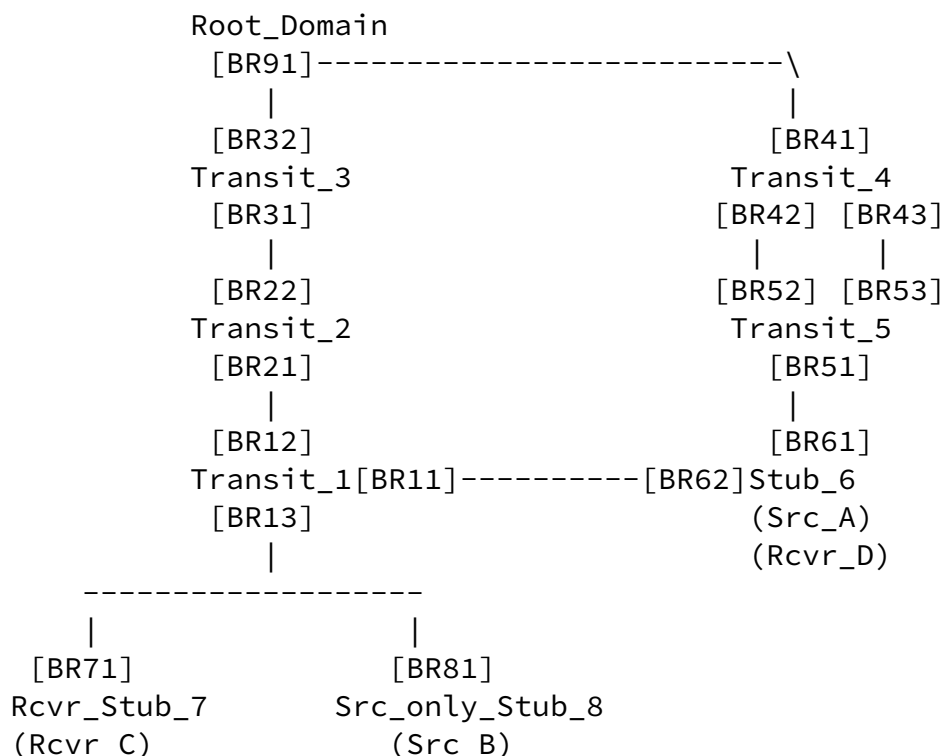
Figure 1: Example inter-domain topology. [BRXY] represents a BGMP border
