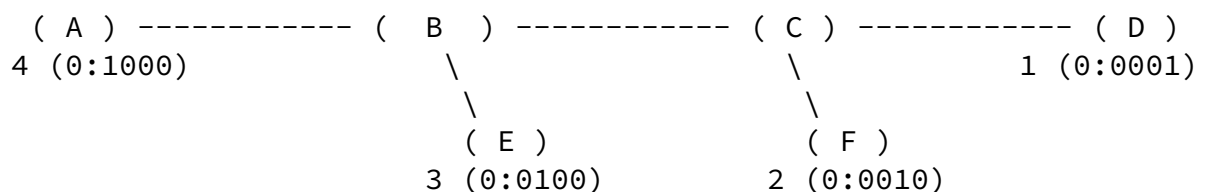
Figure 1: BIER Topology 1
