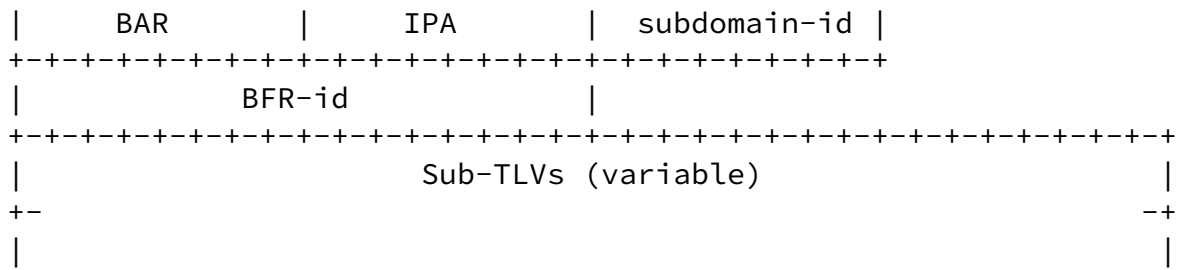
Figure 2: The BIER information TLV
