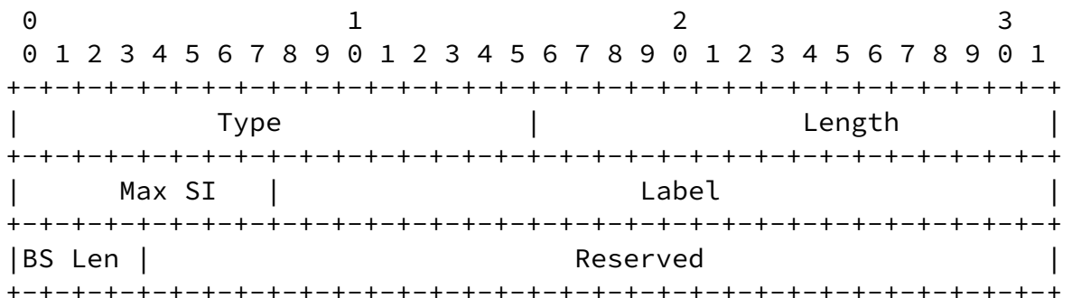
Figure 3: The BIER MPLS Encapsulation TLV
