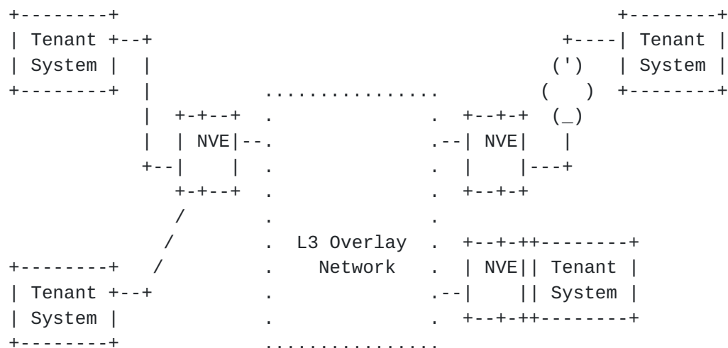
Figure 2: NV03 Architecture
