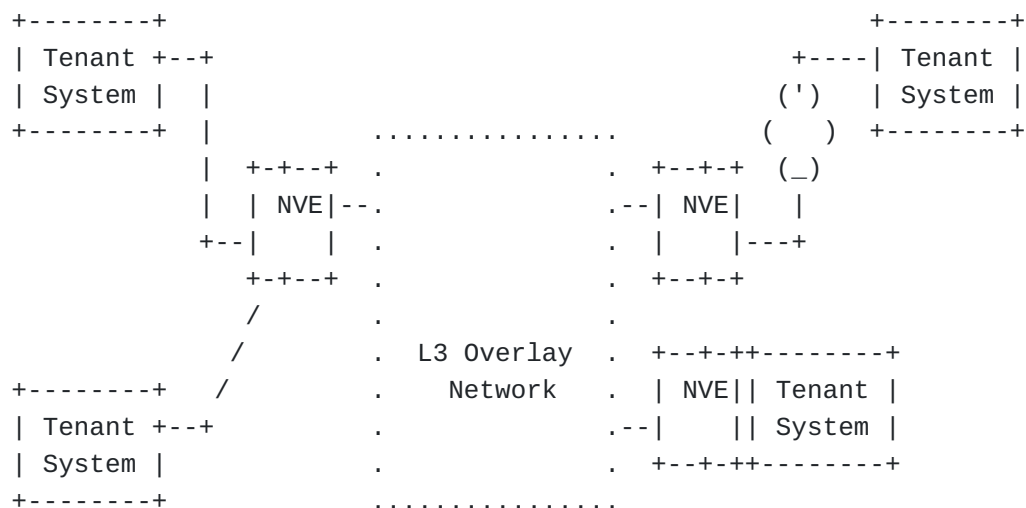
Figure 2: NV03 Architecture
