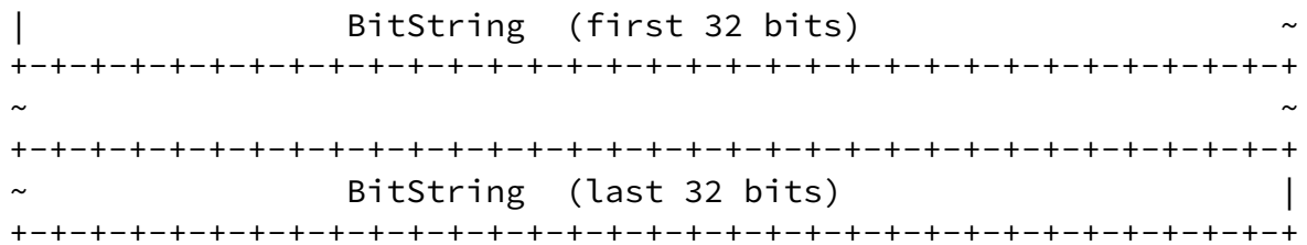
Figure 1: BIER Header
