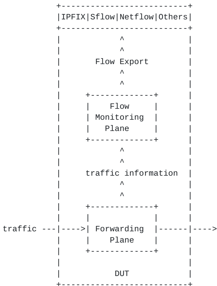
Figure 1. The functional block diagram of the DUT
