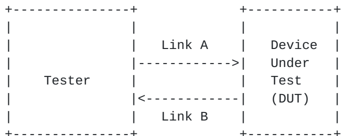
Figure 1: Test Setup
