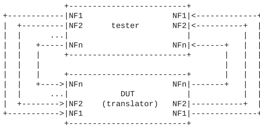
Figure 3. Test setup 3
