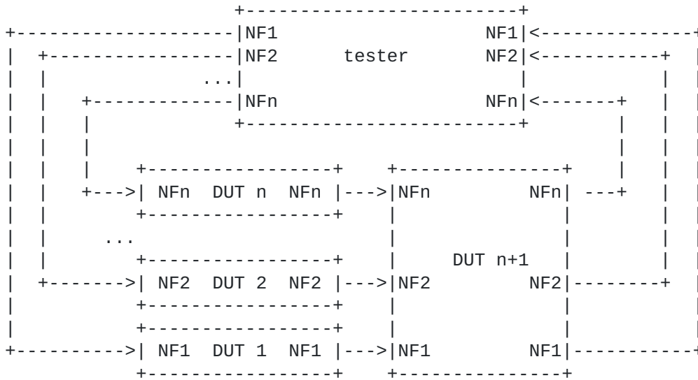
Figure 4. Test setup 4
