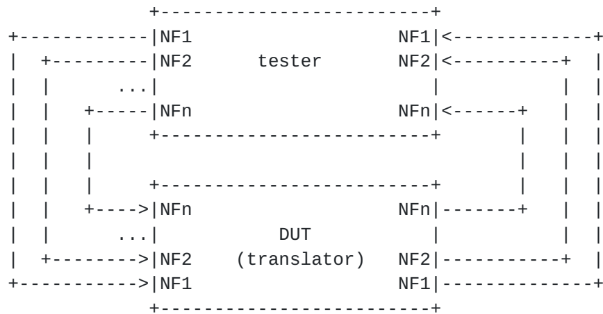
Figure 4. Test setup 3
