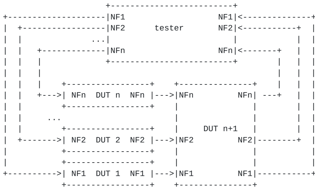
Figure 5. Test setup 4
