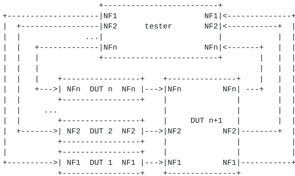
Figure 5. Test setup 4
